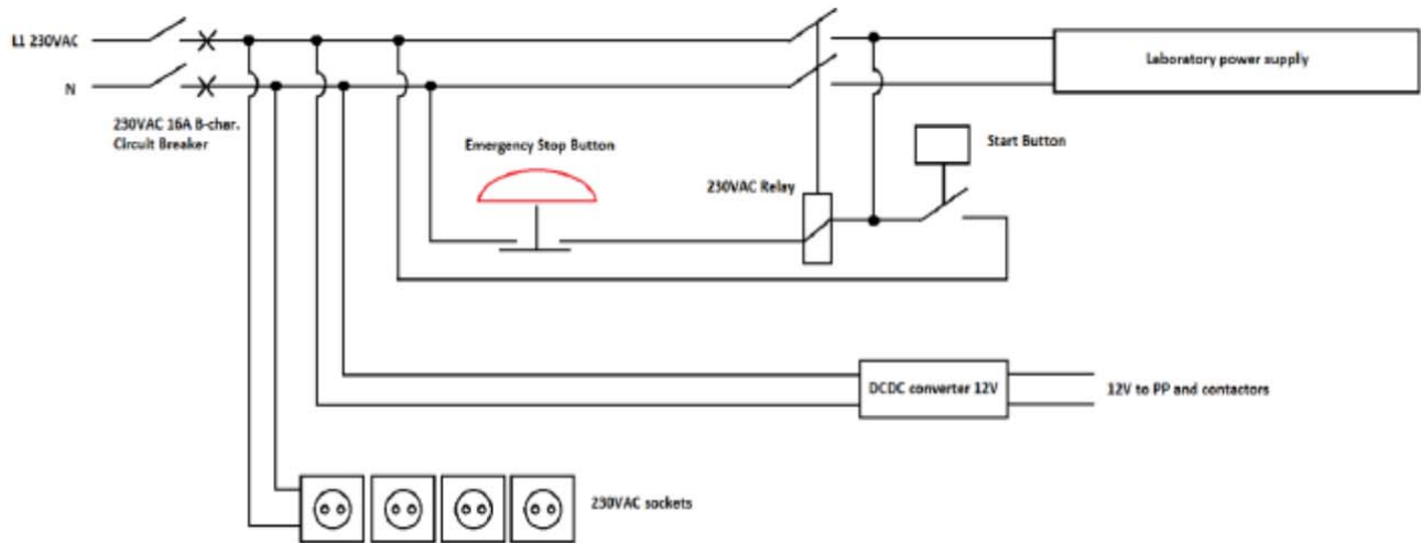
Figure 1: AC electrical setup of DC test benches
