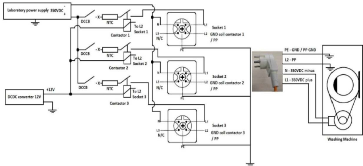
Figure 5: DC electrical setup of DC test benches
