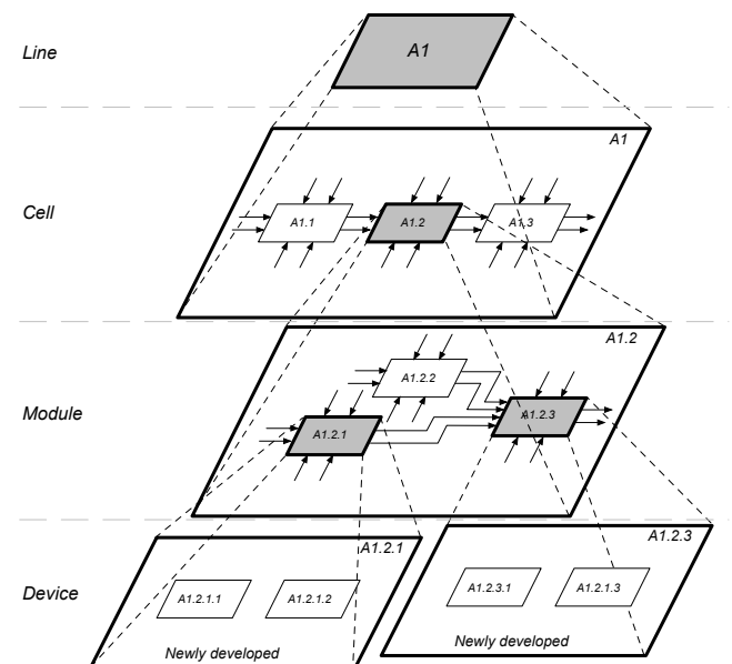
Figure 2: Top down structure of the SADT data-diagram. In a layered structure of Manufacturing- 'Lines', 'Cells', 'Modules' and 'Devices', the structure is decomposed to enable determination which modular parts can be reused or require new development. Changes escalate from bottom to top.
