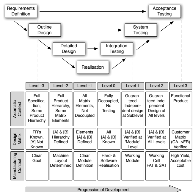
Figure 8: Development of RMSs in seven steps from the embryonic stage to a complete and independent design. Progress again monitored from left to right.
